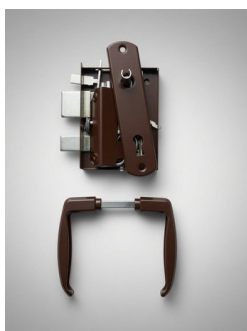
Brown surface-mounted gate lock
